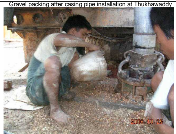
Gravel packing after casing pipe installation at Thukhawaddy
