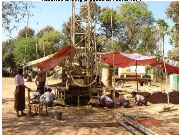
Tubewell drilling process at Tetma no. 1
