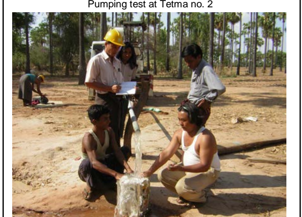
Pumping test at Tetma no. 2
